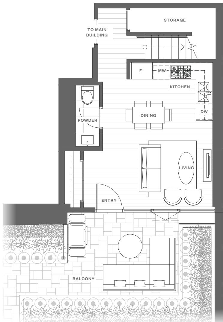
MAIN FLOOR
